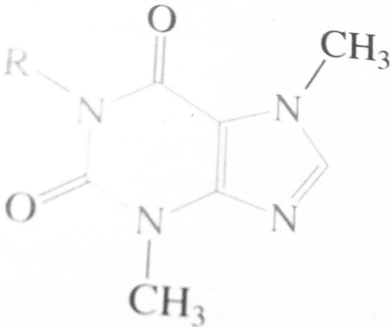
Caféine ( R = CH_3 )
